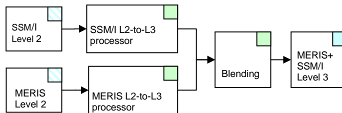
Figure 1: Flow chart of the L3 combined SSM/I+MERIS processor. Products are marked blue (blue shaded: instantaneous level 2 products, blue end product) and software development is marked green.
