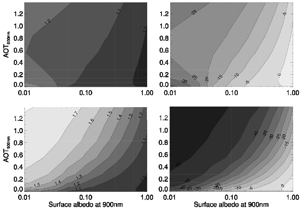
Figure 2: Scattering correction factor f depending on surface albedo and aerosol optical thickness at 900nm (left panels) and equivalent underestimation of TCWV in mm when scattering is neglected (right panels), shown for SZA=64°, VZA=30°, RAA = 0°, TCWV = 56mm and a boundary layer (upper panels) and upper troposphere aerosol layer (lower panels).
