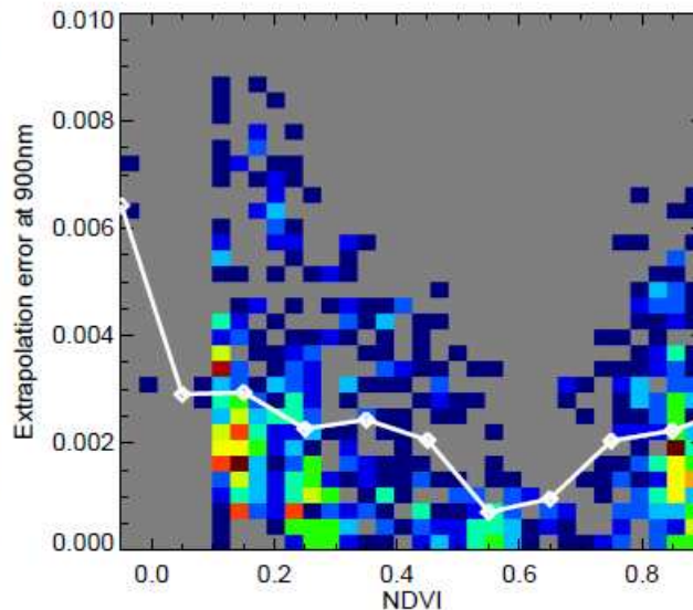
Figure 4: Normalized frequency of occurrence of error of linearly extrapolated surface albedo at 900nm, depending on NDVI and resulting error parameterisation (white curve).
