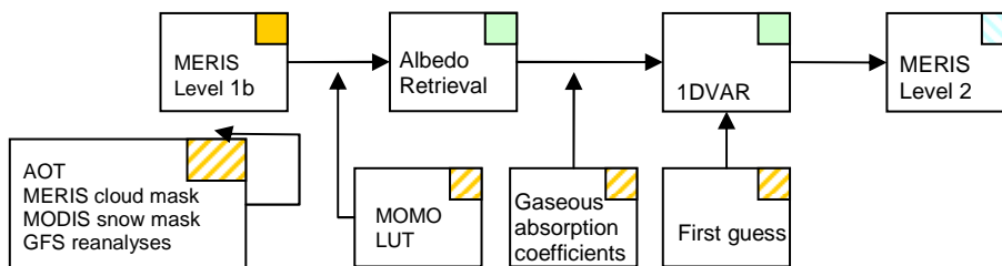
Figure 1: Flow chart for the MERIS L2 processor. Input data is marked in orange (orange shaded: higher level input data), products are marked in blue (blue shaded: instantaneous level 2 products) and software development is marked in green. (GFS: Global Forecasting System, LUT: Look-up table)
