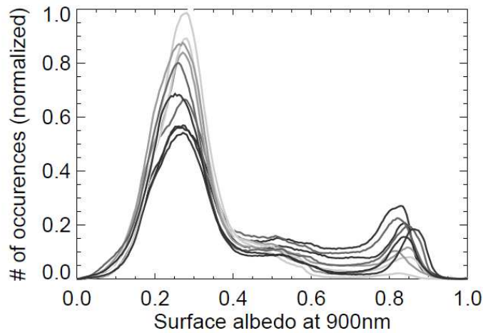
Figure 3: Global, normalized histograms of surface reflectance at 900nm through the year 2004 (grey shading indicating seasonal dependence from winter (dark grey) to summer months (light grey)). Extracted from the MERIS Albedomap.
